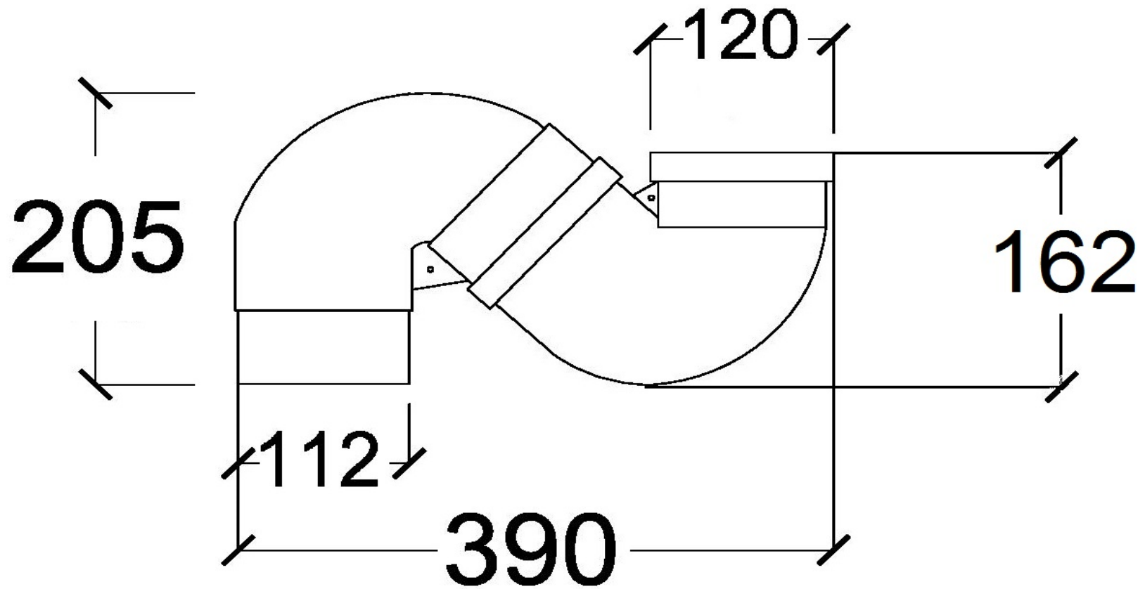
TS390 S TRAP CONNECTOR
