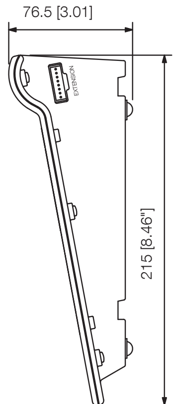
Side View
