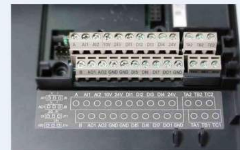
▲ Control circuit terminal
