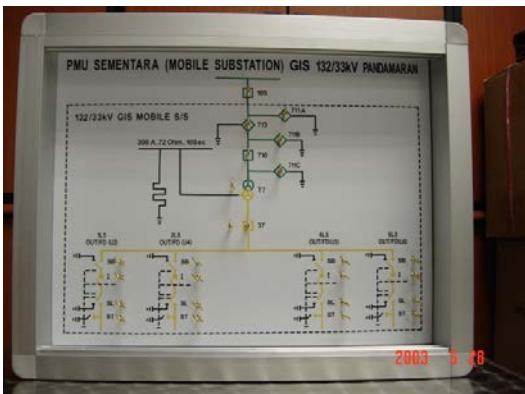
Mobile Substation
