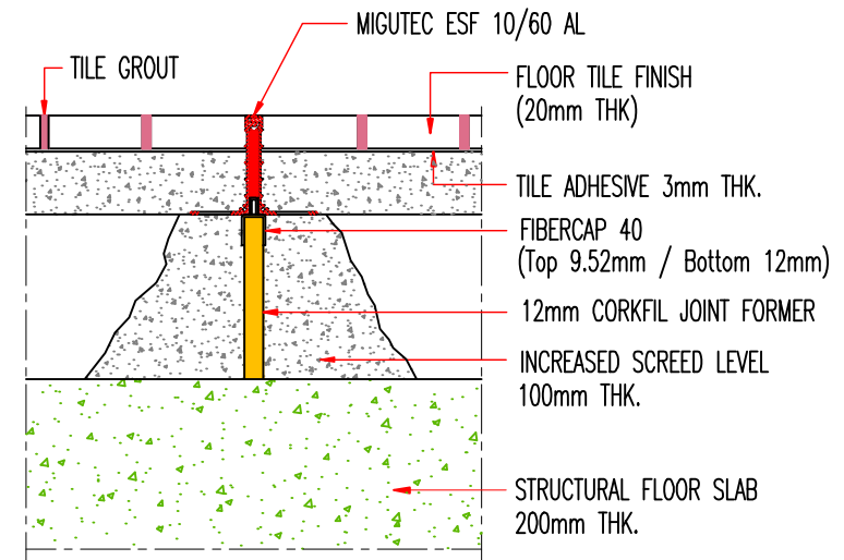
WITH INCREASED LEVELLING SCREED HEIGHT
