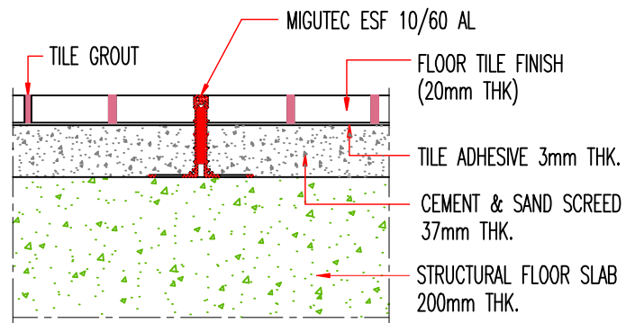
WITH STANDARD SCREED LEVELLING HEIGHTS
