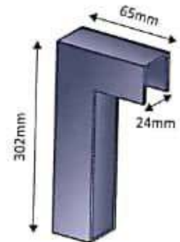
90° Corner joint and Hinges Bracket
