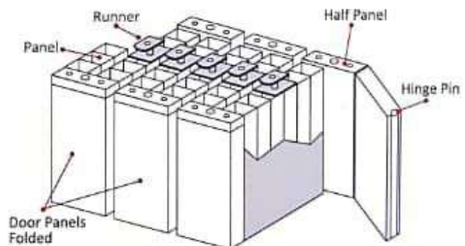
Structure Section A-A
