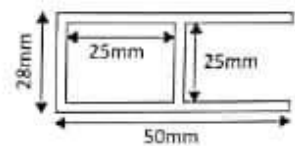
Extruded PVC Solid Panel Frame
