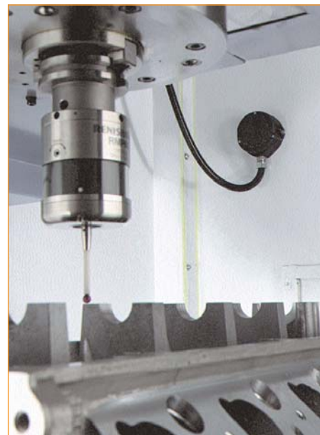
RMP60 probe inspecting a component, with RMI receiver / interface in the background
