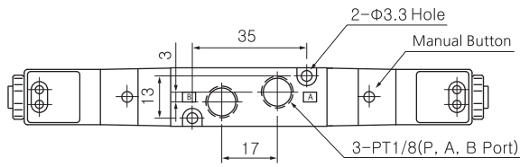
2position / 5port double(Grommet type)
