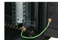
Earthing cable
