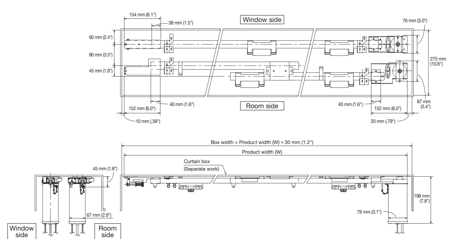
Straight: ceiling double attachment (Room side: Rail overlap, Window side: Master roller)
