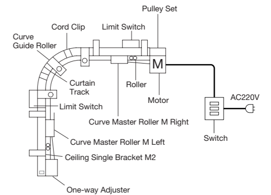
Curve: Two-way draw (Master roller)
