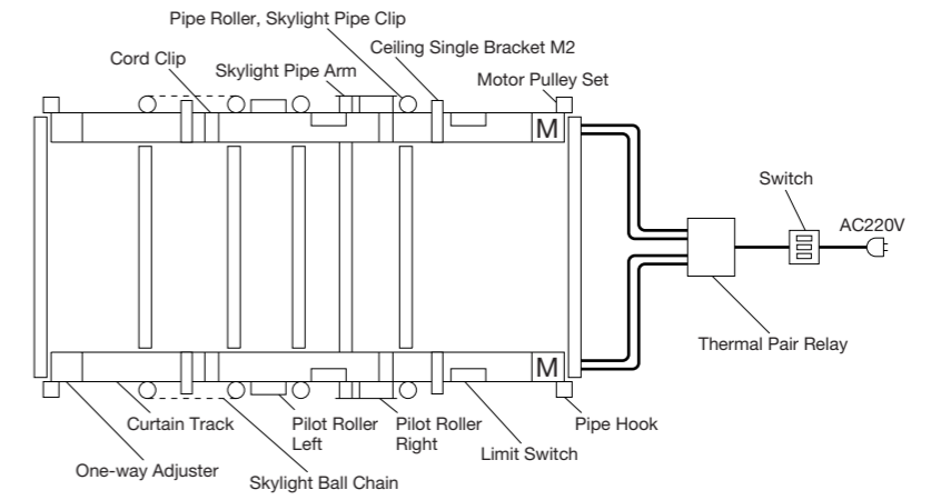
Skylight and Slope skylight: Two-way draw
