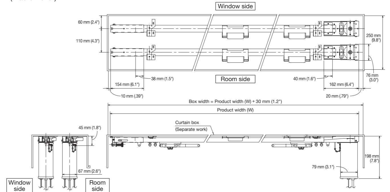
Straight: ceiling double attachment (Master roller)
