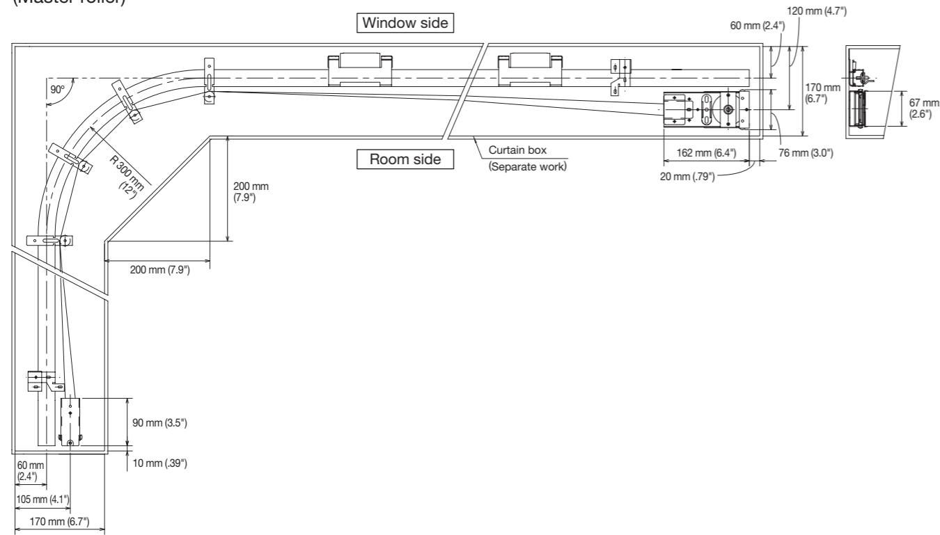
Curve: ceiling single attachment (Master roller)
