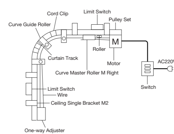
Curve: One-way draw
