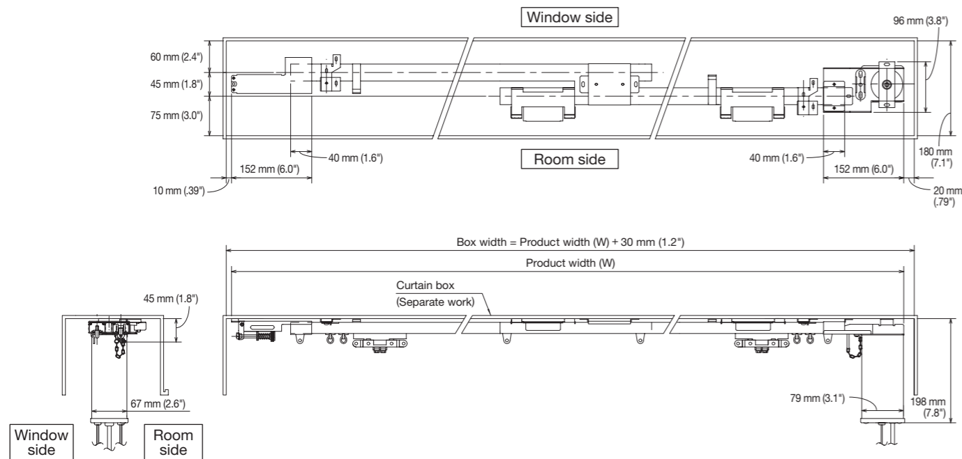
Straight: ceiling single attachment (Rail overlap)
