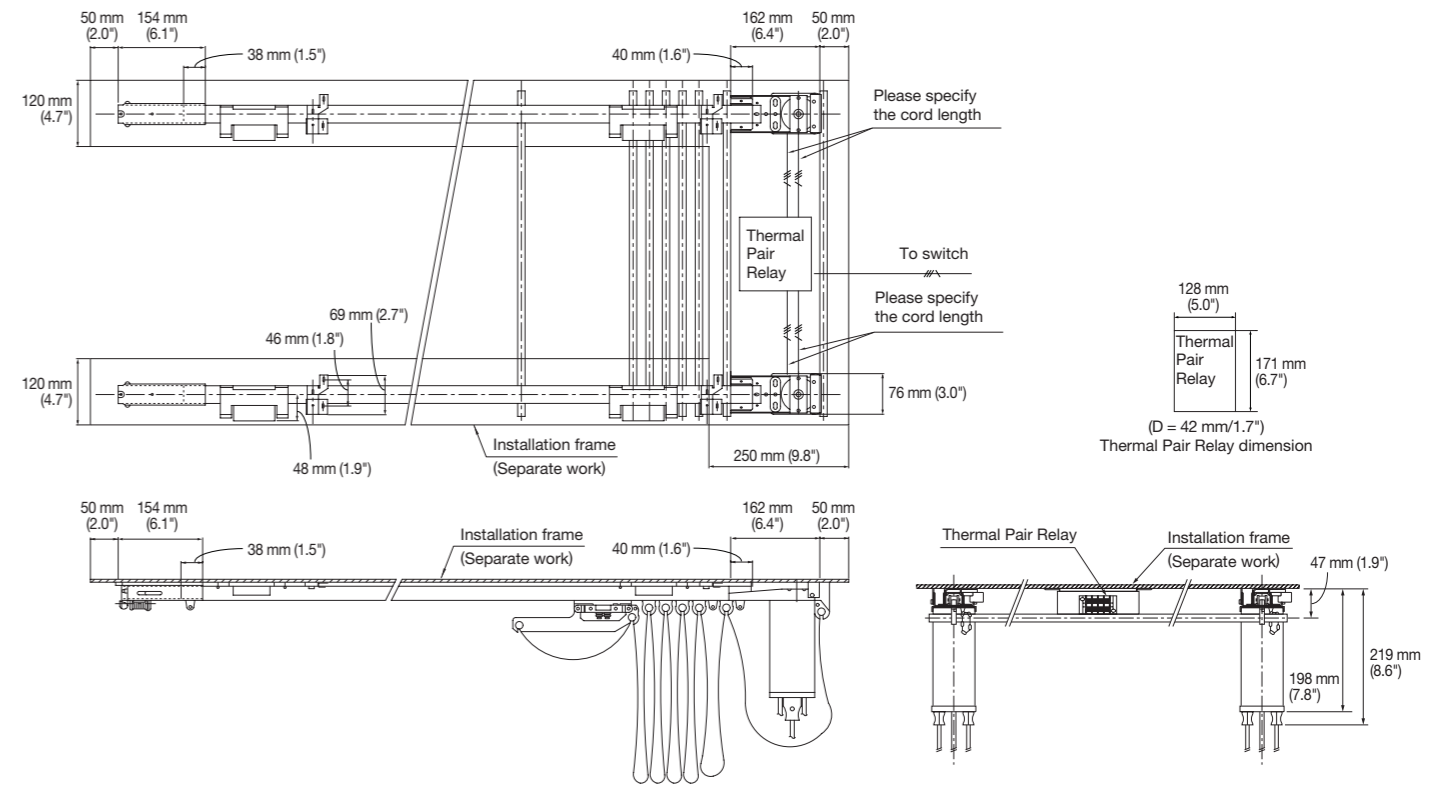
Skylight, Slope skylight: Two-way draw
