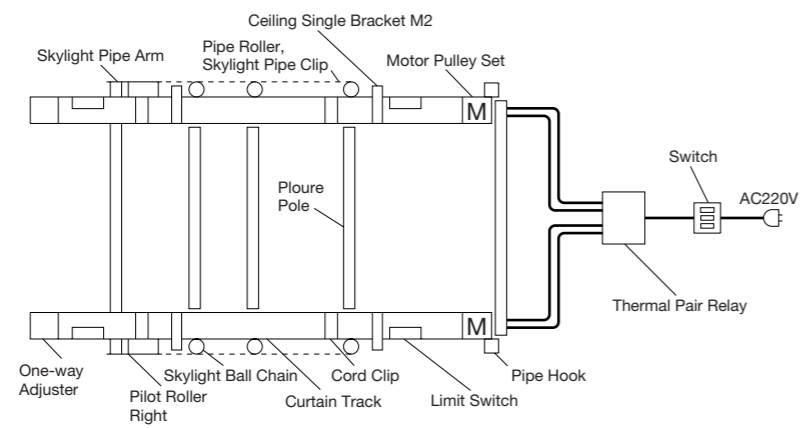
Skylight and Slope skylight: One-way draw
