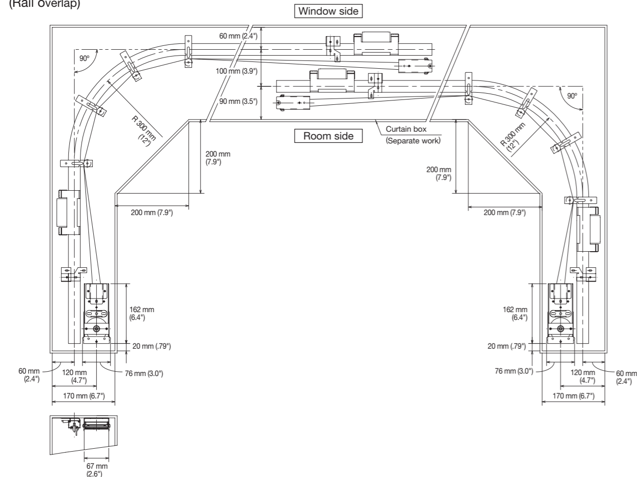
Curve: ceiling single attachment (Rail overlap)
