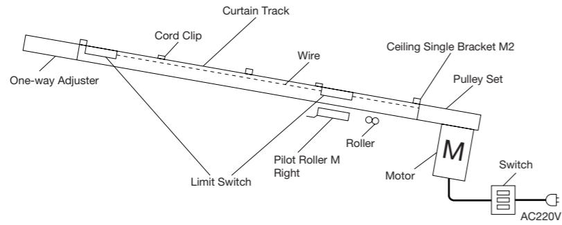
Slope window: One-way draw
