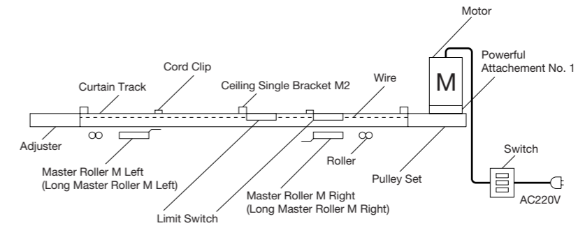
Straight: Two-way draw (Motor recessed in ceiling)
