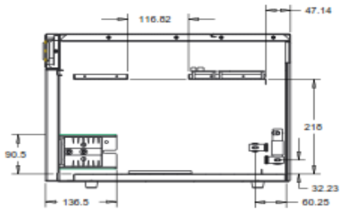
SECTION A-A SHOWN WITHOUT MODULES
