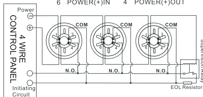
4 wire detectors wiring diagram
