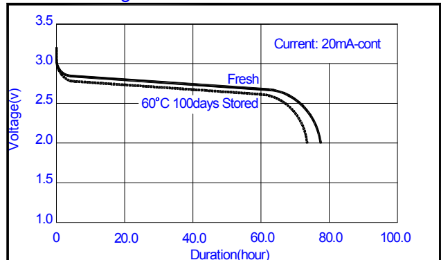
Discharge Characteristics
