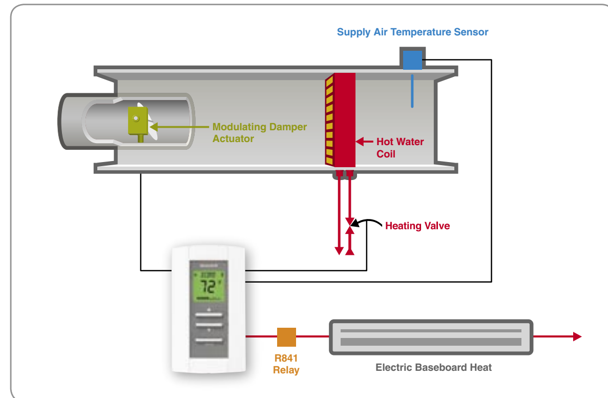
TB7980B1005: Pressure Dependent VAV Cooling With Zone Reheat and Electric Baseboard Heat
