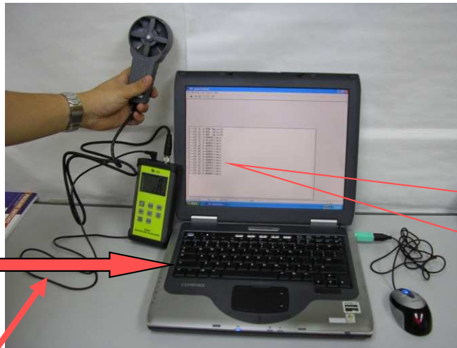
TPI 575C1 is communicating with Computer via A500 Cable + Hyper Terminal = Datas
