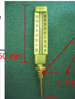
Thermometer
