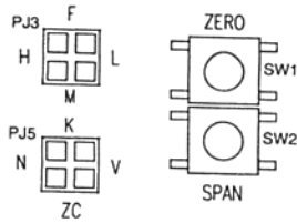
Figure 5: Mode and Range Programming Jumpers and Switches
