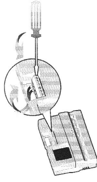
Fig. 5. Connect system wires to thermostat terminals (strip 5/6 inch).
