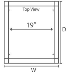
Dimension For 19" Wall Mount
