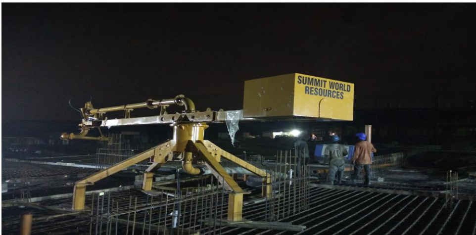
Figure 2: Summit World Resources' KRV10 during casting
