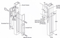
Dimension of J5, J6 & J7
