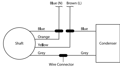
Top View of Motor Terminal
