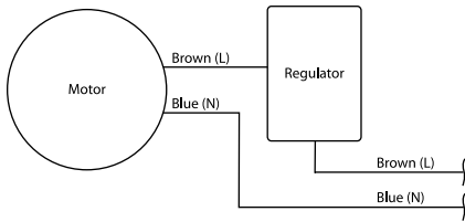
Connection Diagram
