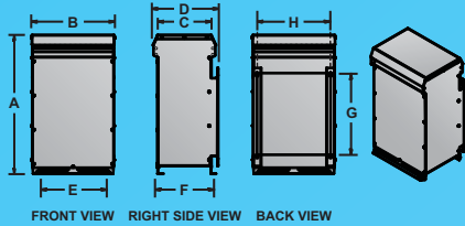
'SU' ENCLOSURE
