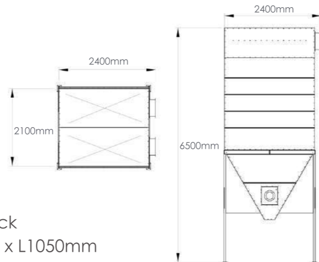
Dust Collector
