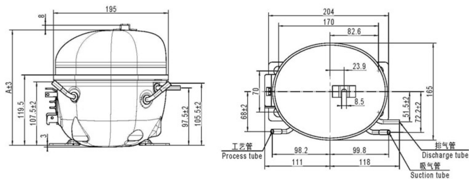
W 系列外观 W Series External Views
