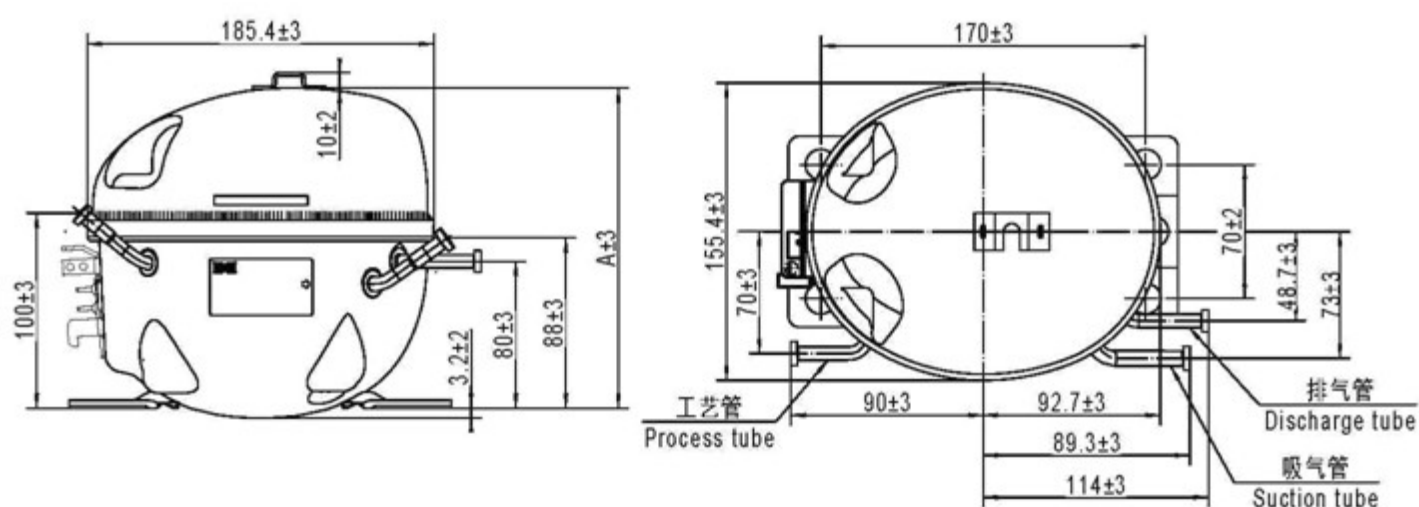
T 系列外观 T Series External Views
