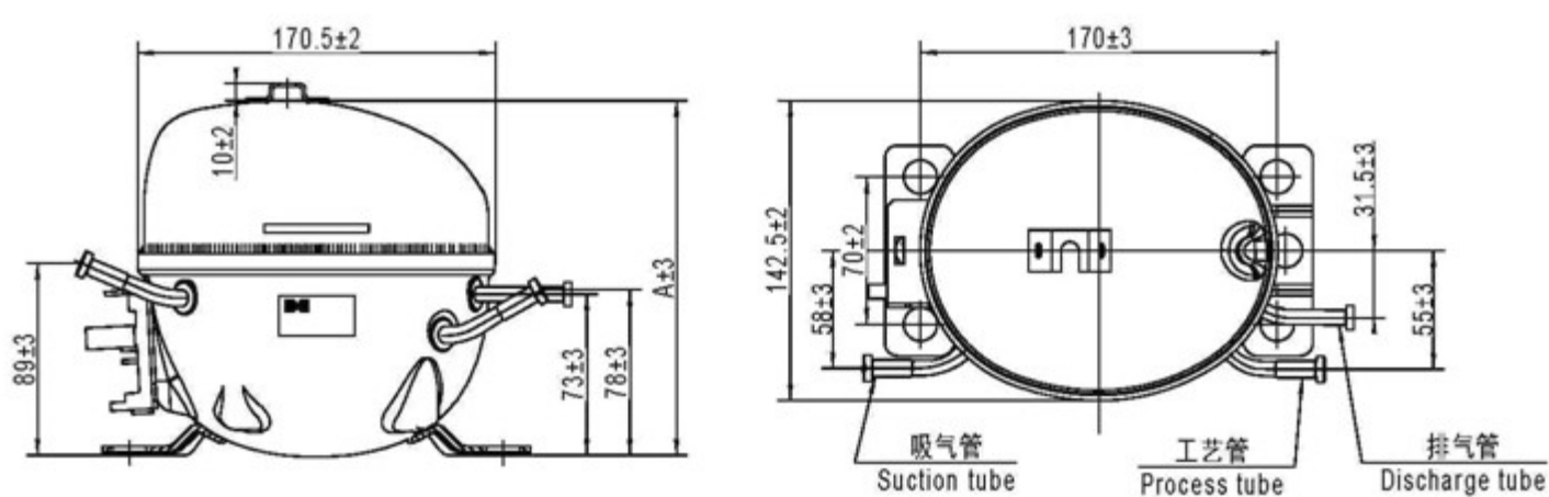
S 系列外观 S Series External Views
