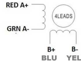
Bi-Polar Connection
