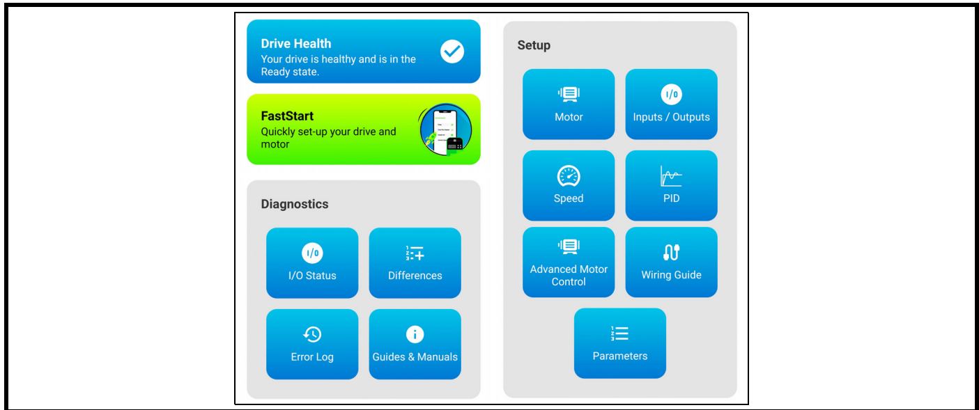
Figure 5-2 Marshal dashboard
