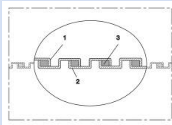
Metal hose, stainless steel (INOX), suction hose (up to +600°C)
