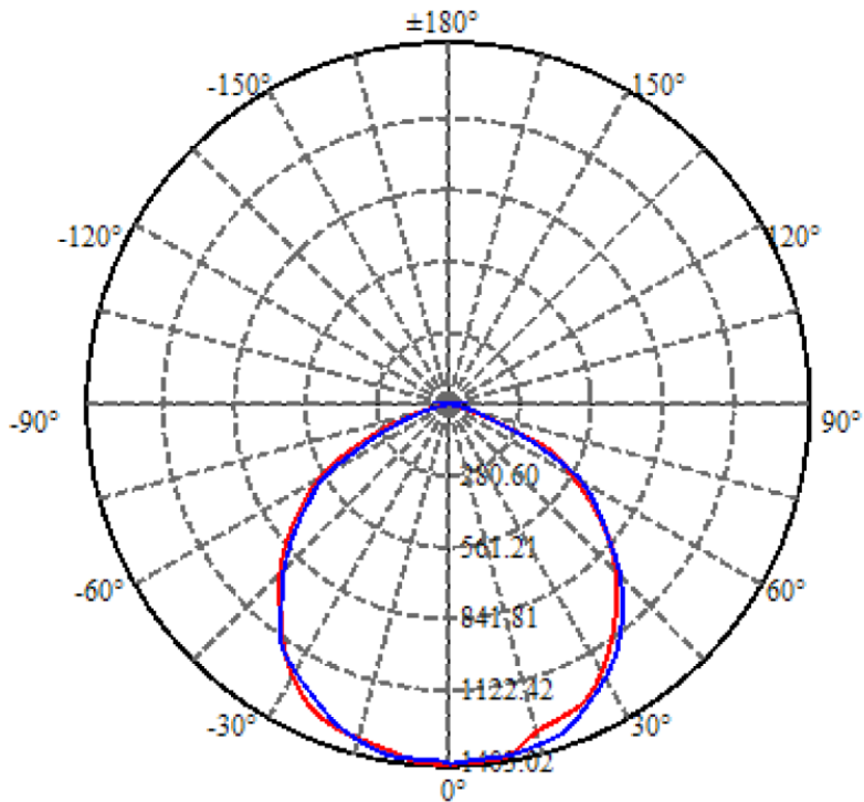
Isocandela diagram
