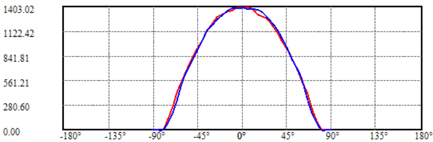
Cartesian coordinates
