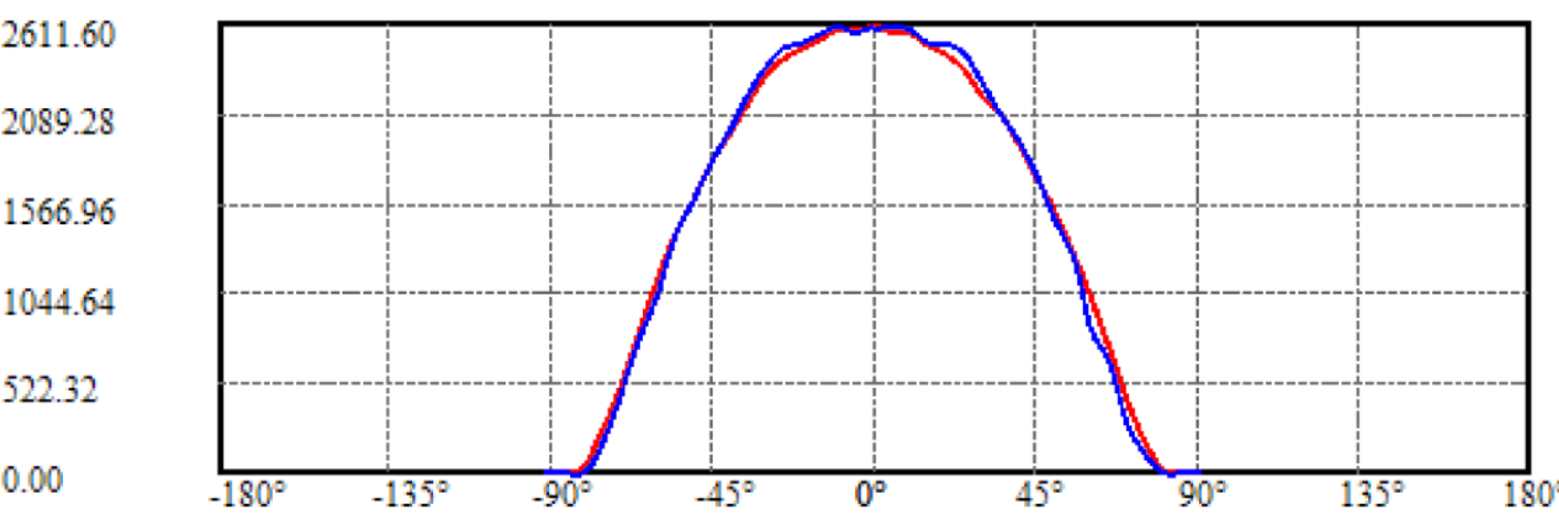
Cartesian coordinates
