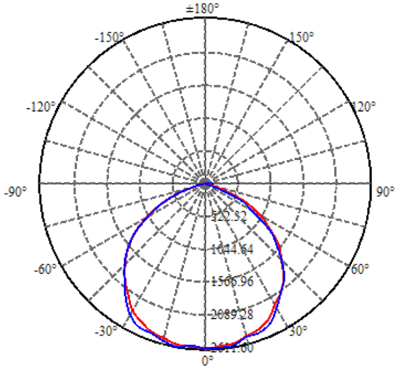
Isocandela diagram
