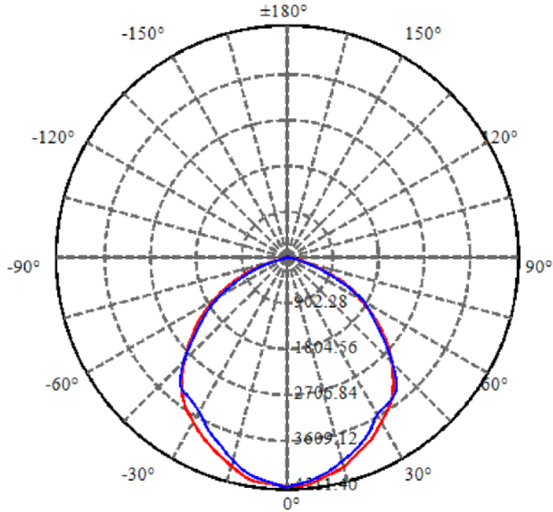
Isocandela diagram
