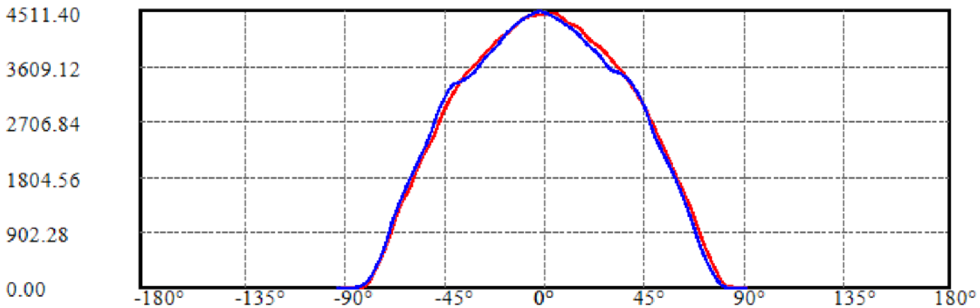
Cartesian coordinates
