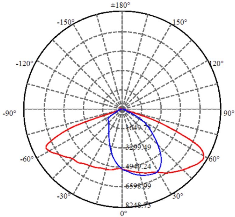
Isocandela diagram
