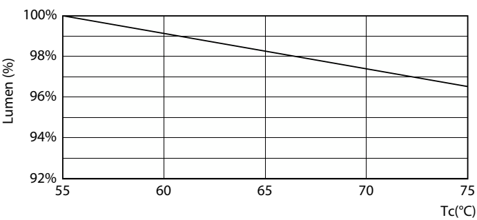
Lumen Maintenance Diagram - Ecofit E LEDtube 1200mm 18W 740 T8 I MY
