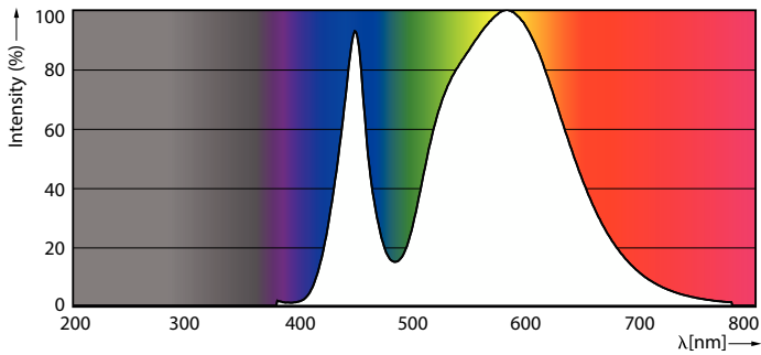
Spectral Power Distribution Colour - Ecofit E LEDtube 1200mm 18W 740 T8 I MY
