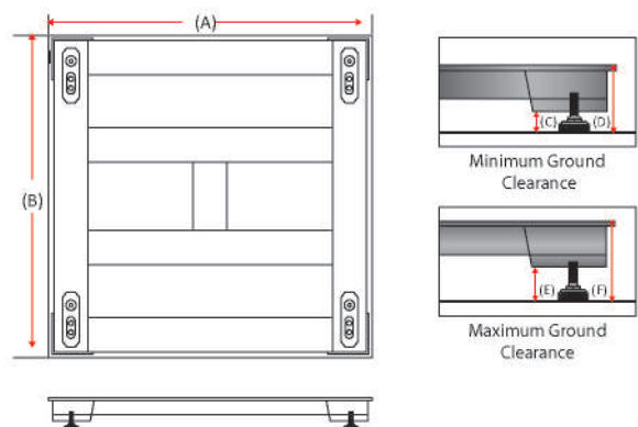
Dimension of digital floor scale in mm
