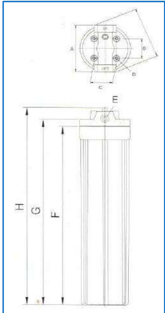
Figure 3 : Dimensions for SYSFLO CB Series Plastic Filter Housing
