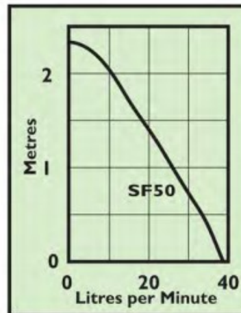
Max head 2.3 M - Max flow 38 lpm
