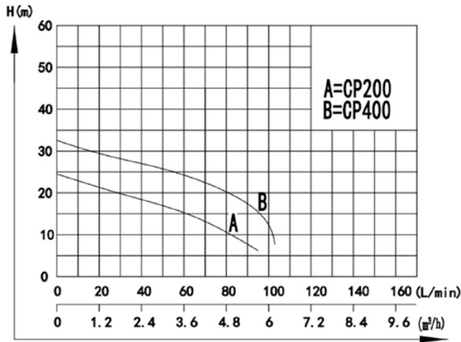
Pump Performance
