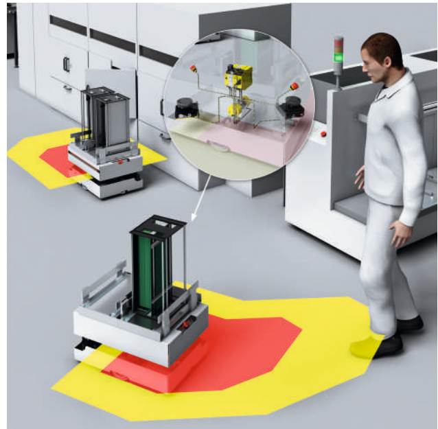
Figure 65: Application example for protective fields on an autonomous vehicle
