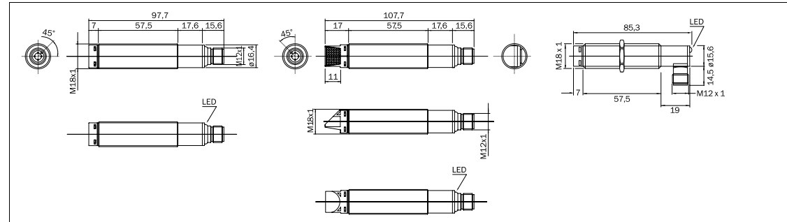
Abb. 6: L41X-21XA1A
