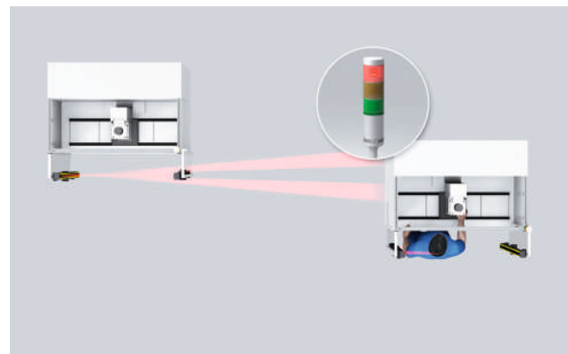
Figure 53: No mutual interference of protective devices due to suitable arrangement of the machine or ESPE systems
