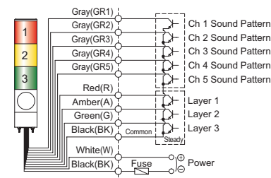
EXTERNAL TRANSISTOR-NPN
