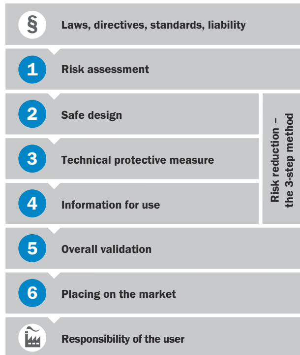
Figure 2: Structure: “Six steps to a safe machine”
