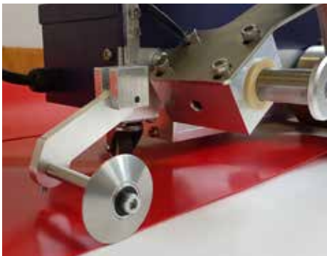
Track guide roller for more accuracy
