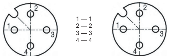
Fig. 8 Pin assignment for the Flex version
