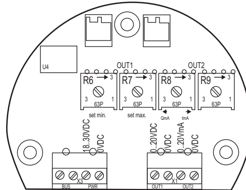
Fig. 6 Adjusting potentiometers
