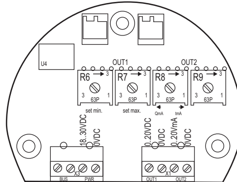
Fig. 7 Connection diagram
