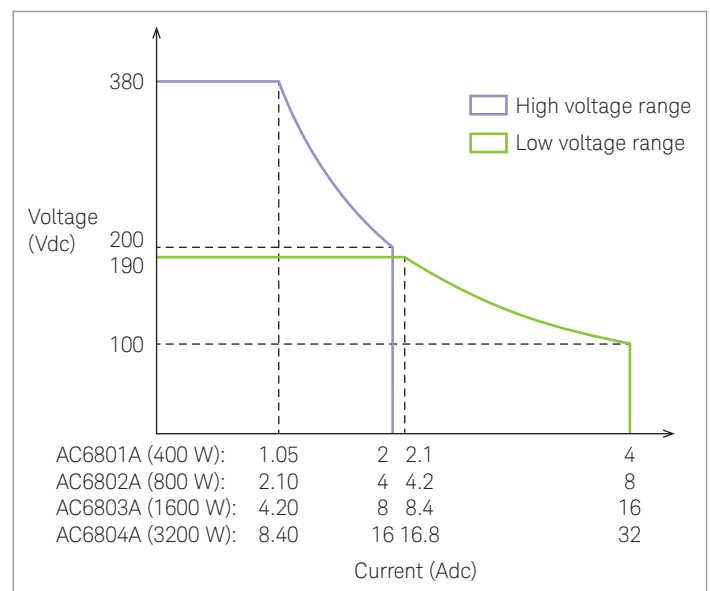
AC6800 steady-state DC output characteristic
