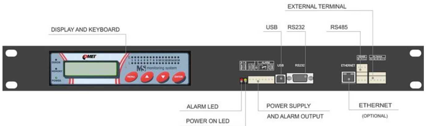
Figure: communication interface, alarm outputs, connection of power. Ethernet interface is optional.
