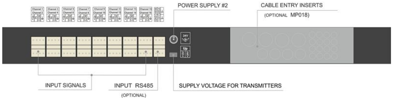
Figure: inputs panel with a voltage selector 12Vdc/24 to power the connected sensors. Serial input RS485IN is optional.
