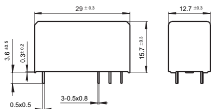
3.5mm Pinning (HF115F/□□□-□□-□-1-□□)
