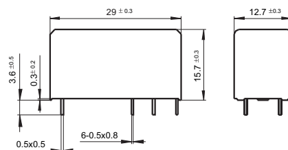
5mm Pinning (HF115F/□□□-□□-□-2/3/4-□□)
