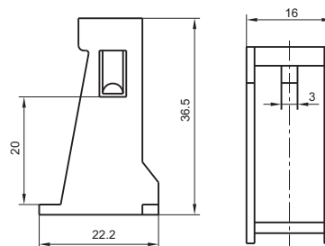
140F-H1(Plastic retainer)
