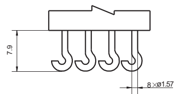
Terminal style 4 (Solder hook)
