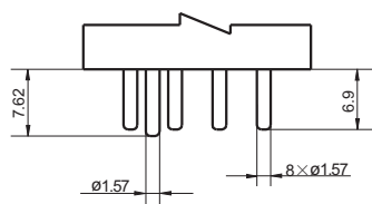
Terminal style 2 (Solder pin)
