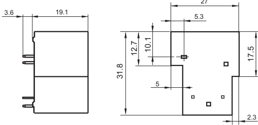
Outline Dimensions
